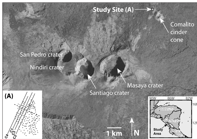
Figure 1. Aerial photograph showing study site location adjacent to Comalito cinder cone on the flanks of Masaya volcano. Inset (A) shows locations of inferred normal fault (dashed line), 2002 measurement locations (dots), and transects C1–C4.
