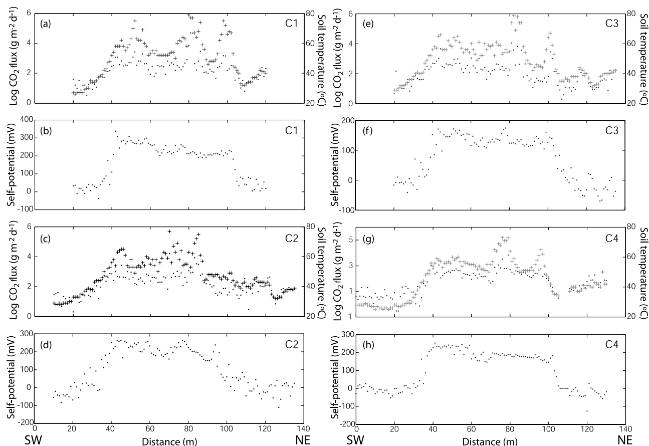
Figure 3. Plots of log CO 2 flux and soil temperature versus distance along transects (a) C1, (c) C2, (e) C3, and (g) C4 (see Figure 2). Dots and pluses are log CO 2 flux and soil temperature, respectively. Plots of SP versus distance along transects (b) C1, (d) C2, (f) C3, and (h) C4.
