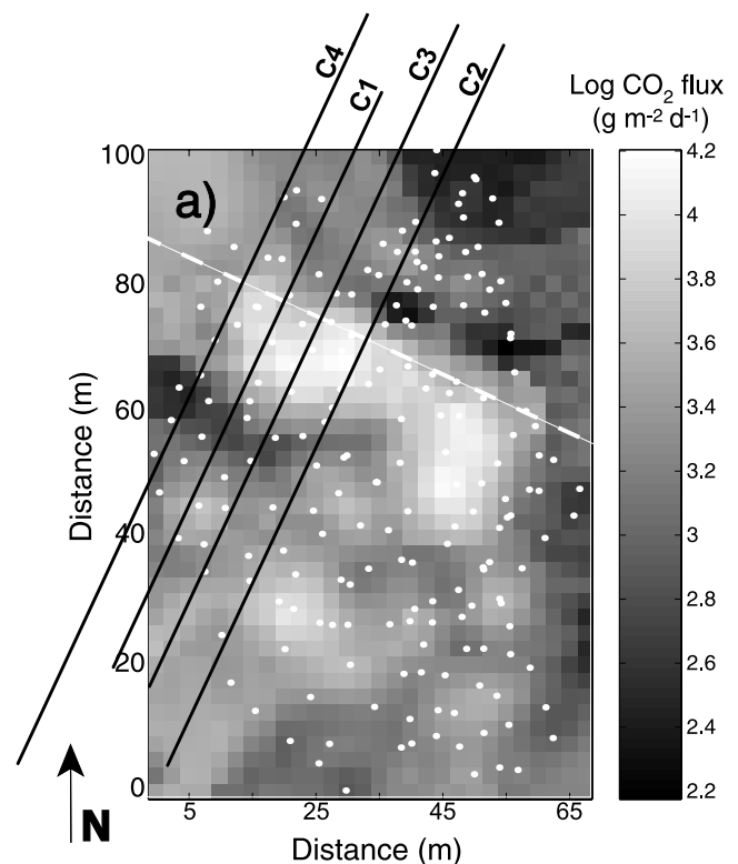
Figure 2. Interpolated (Kriging method) image map of log \text{CO}_2 flux measured adjacent to Comalito cinder cone. White dashed line and dots show locations of inferred normal fault and soil \text{CO}_2 flux and temperature measurements (temperature data not shown), respectively. Also shown are locations of transects C1–C4.
